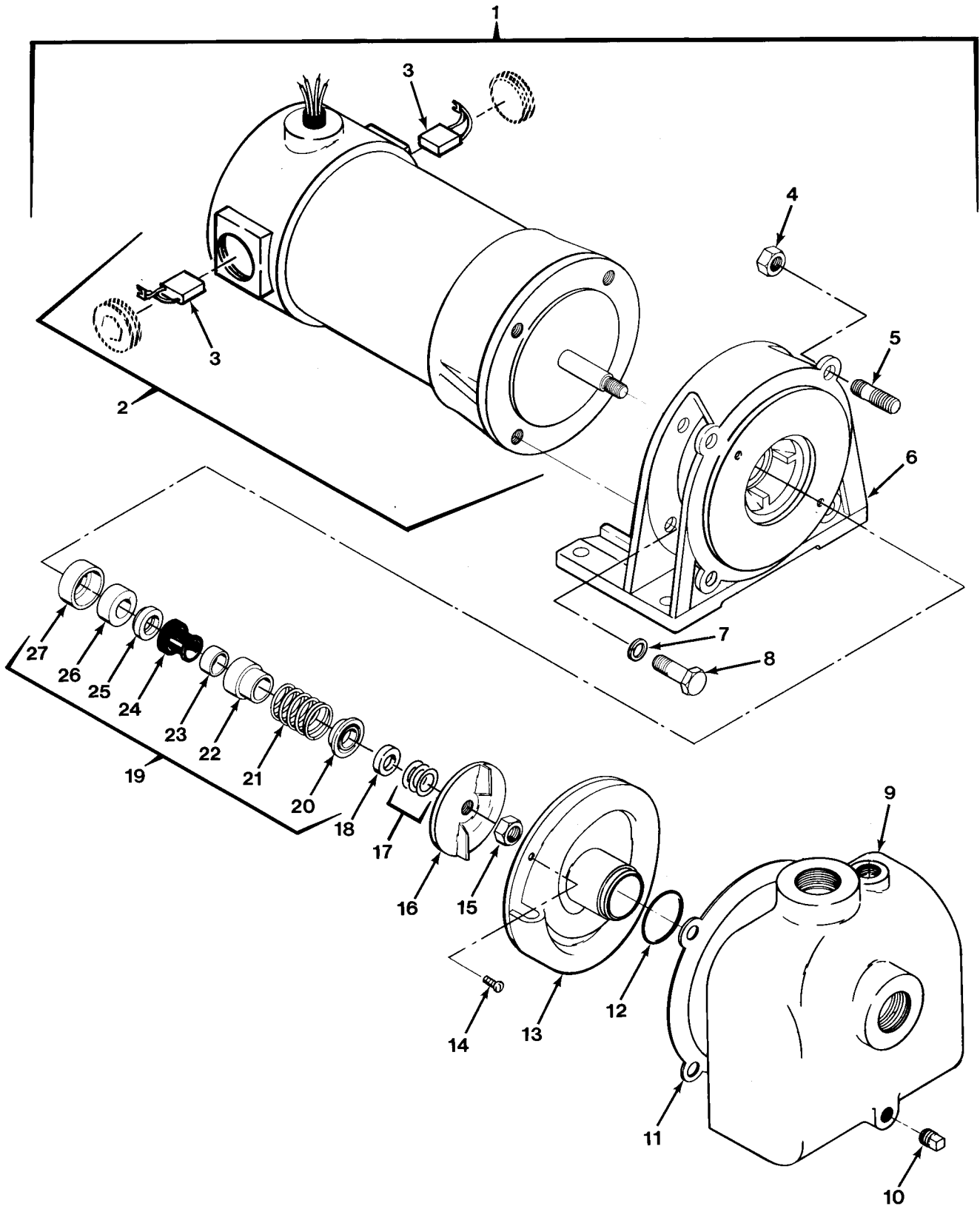
FIG.444 AUXILIARY PUMP
