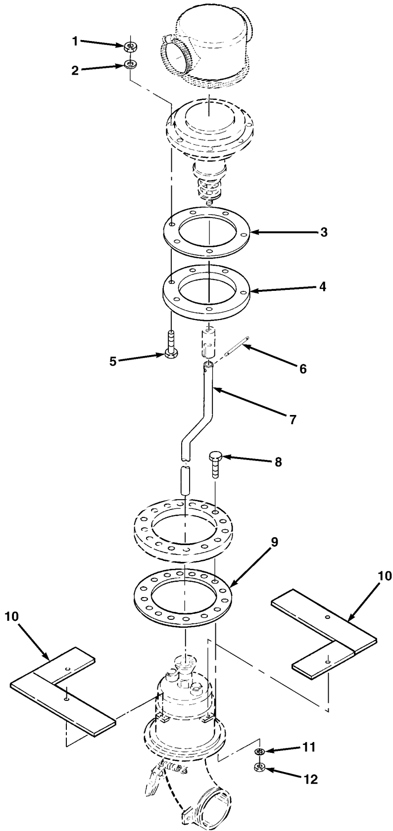
FIG.455 V10 BOTTOM LOAD INSTALLATION
